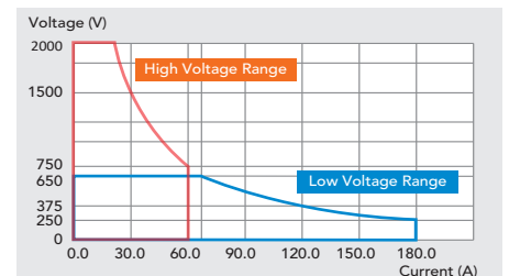
62450D-2000HL操作范围 (Source Mode)
