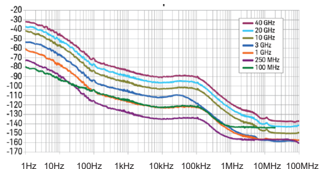
L(f) [dBc/Hz] 与频率 [Hz]
