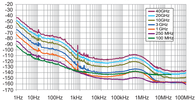
L(f) [dBc/Hz] 与频率 [Hz]
