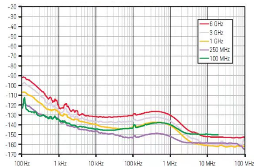
L(f) [dBc/Hz] 与频率 [Hz]
