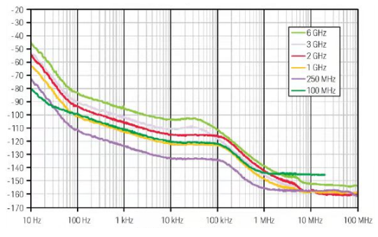
L(f) [dBc/Hz] 与频率 [Hz]
